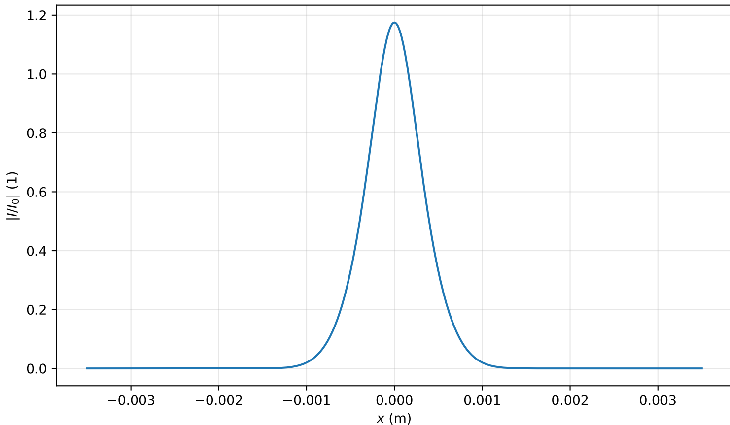
Intensity profile I(x, y = 0, z = 0.557m)/I_0 , P_{in}=0.9P_{cr} , artificial time
